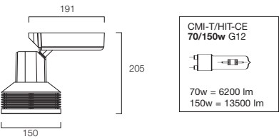
Housing + Reflector
