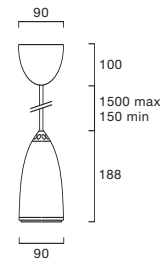
Hi-Spot ES50
